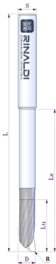
AL1ARS
